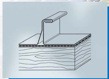
Angle lock-welt Used primarily for wall claddings
