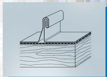
Double lock-welt Suitable for roofing and wall cladding
